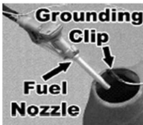
Fuel Nozzle in contact with receiving tank
