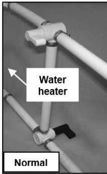
Two Valve Water Heater Bypass
