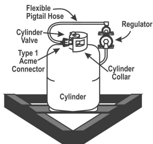
Single Cylinder
