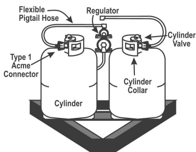
Double Cylinder
