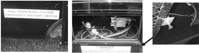
Master/Emergency Fuel Disconnect Switch locations
