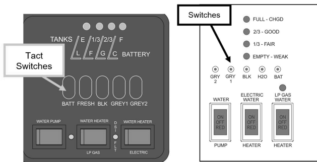
Command Center Panel
